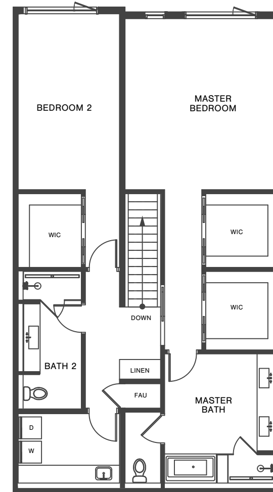
SECOND LEVEL
