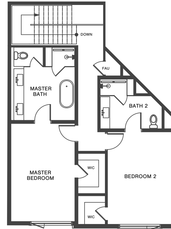
SECOND LEVEL
