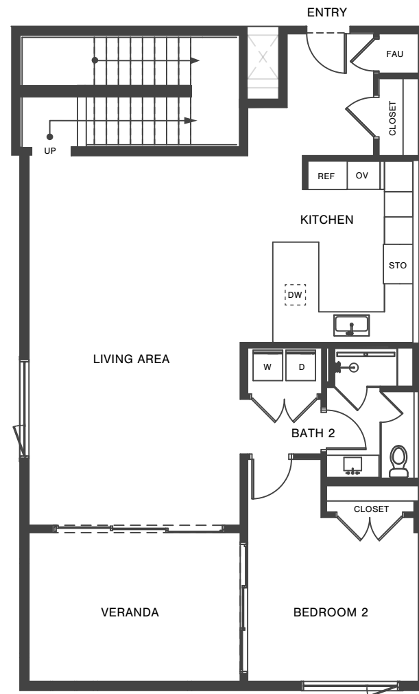
FIRST LEVEL
